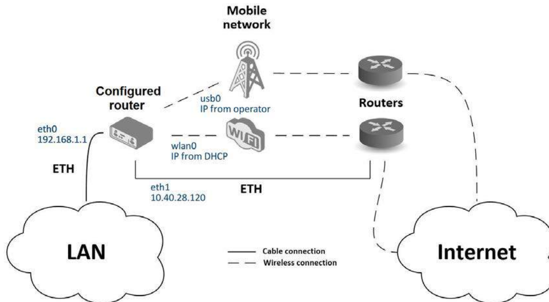
Figure 92: Backup access to the Internet – sample topology
