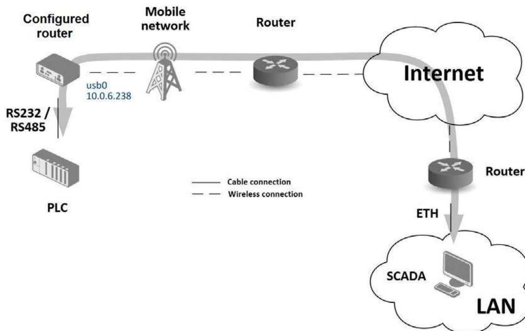
Figure 99: Serial Gateway – sample topology
