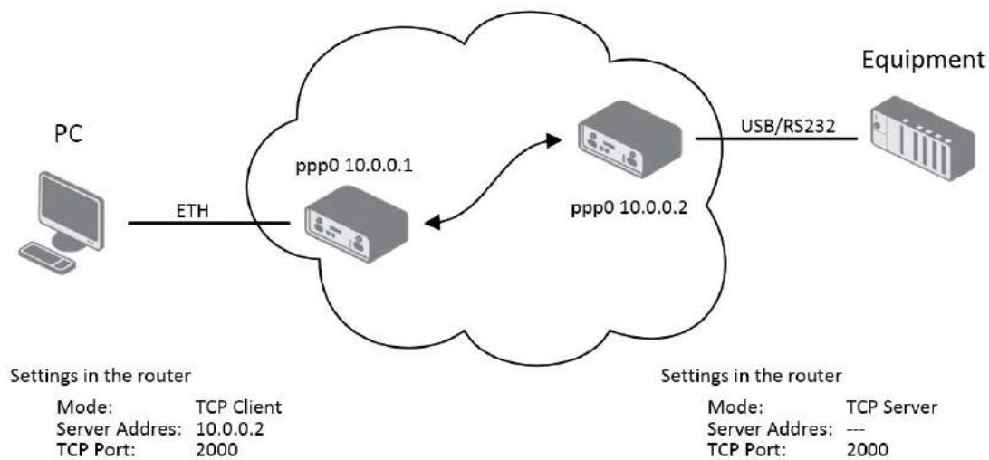
Figure 70: Example 2 – USB port configuration
