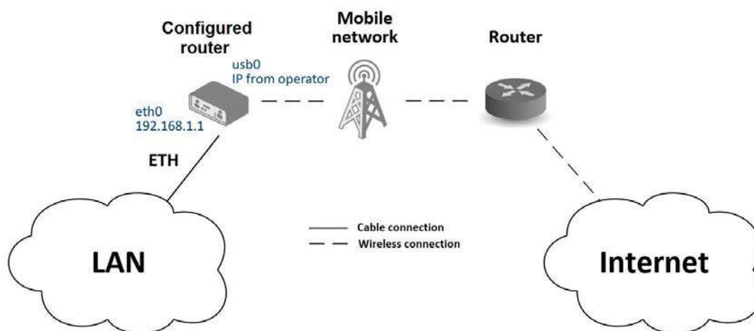
Figure 89: Access to the Internet from LAN – sample topology
