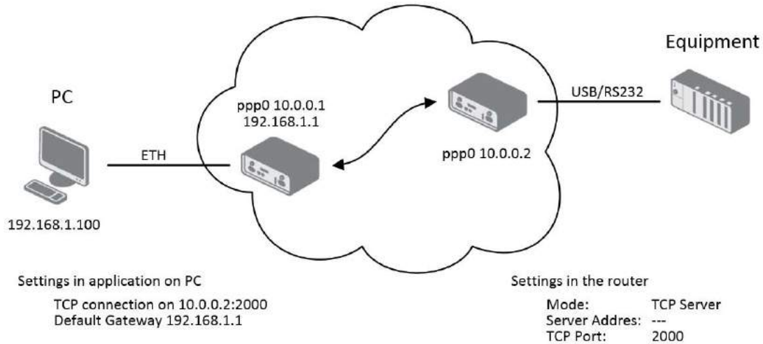
Figure 69: Example 1 – USB port configuration
