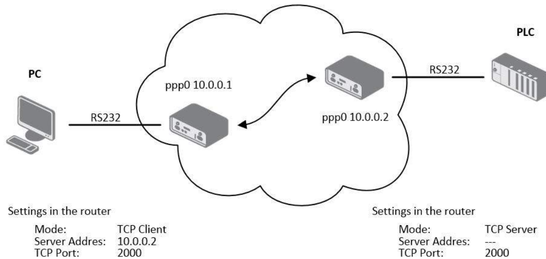
Figure 67: Example of serial interface configuration
