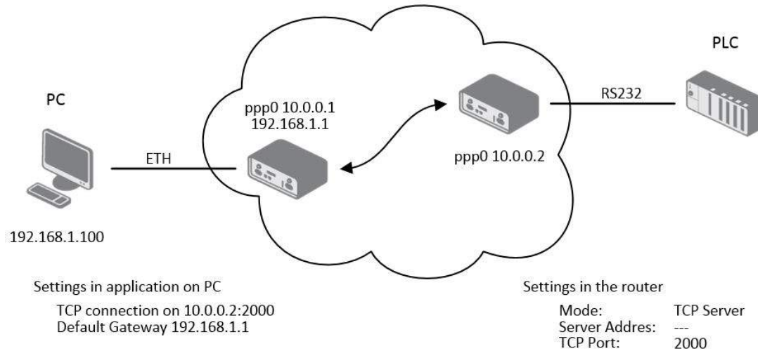
Figure 66: Example of Ethernet to serial communication configuration
