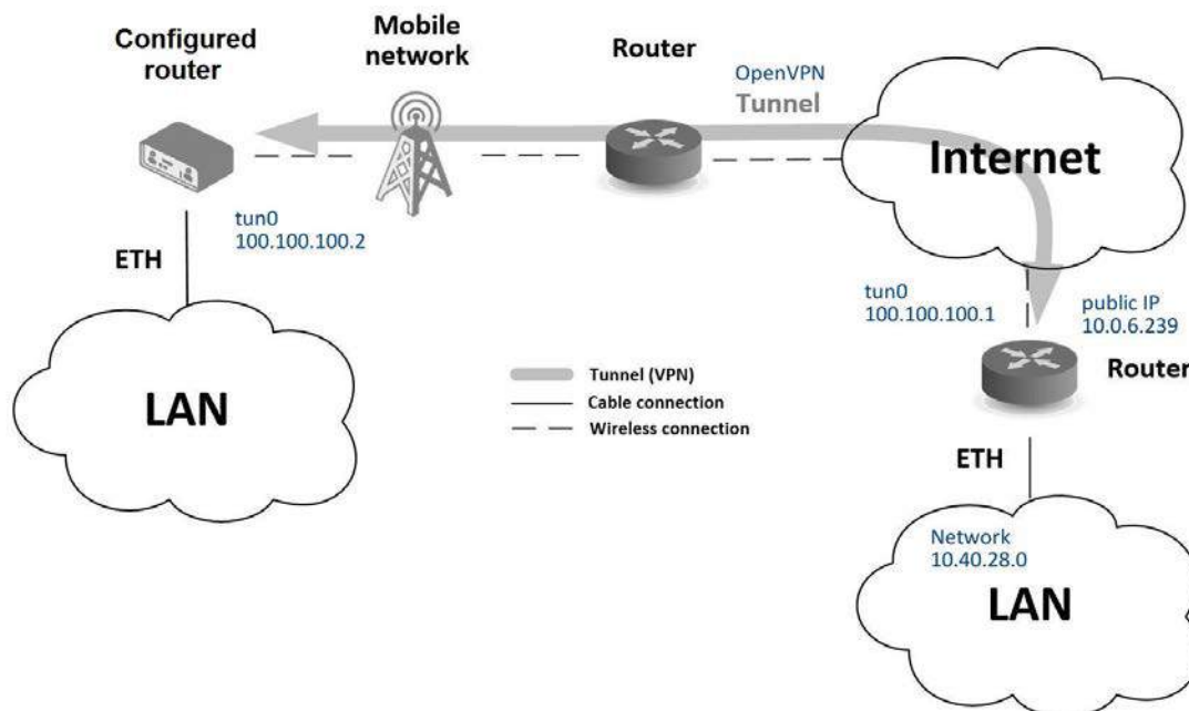
Figure 97: Secure networks interconnection – sample topology
