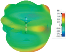
3D Plot Element C Top (2600 MHz)
