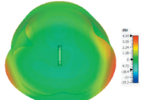
3D Plot Element B Side (2600 MHz)
