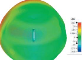
3D Plot Element A Side (2600MHz)
