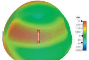
3D Plot Element D Side (2600 MHz)
