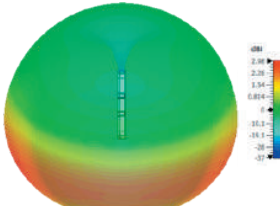
3D Plot Element C Top (850 MHz)
