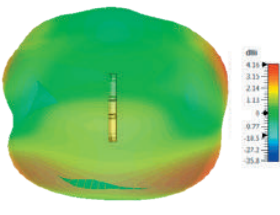
3D Plot Element C Top (2600 MHz)
