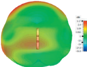
3D Plot Element A Top (2600MHz)
