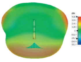
3D Plot Element C Side (2000 MHz)
