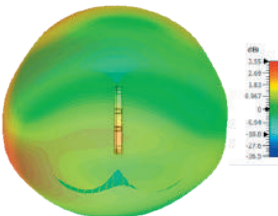
3D Plot Element A Side (2000MHz)
