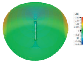
3D Plot Element A Top (850 MHz)
