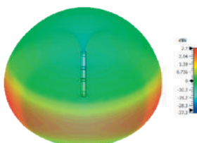
3D Plot Element C Top (1800 MHz)
