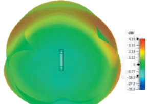
3D Plot Element C Side (2600 MHz)
