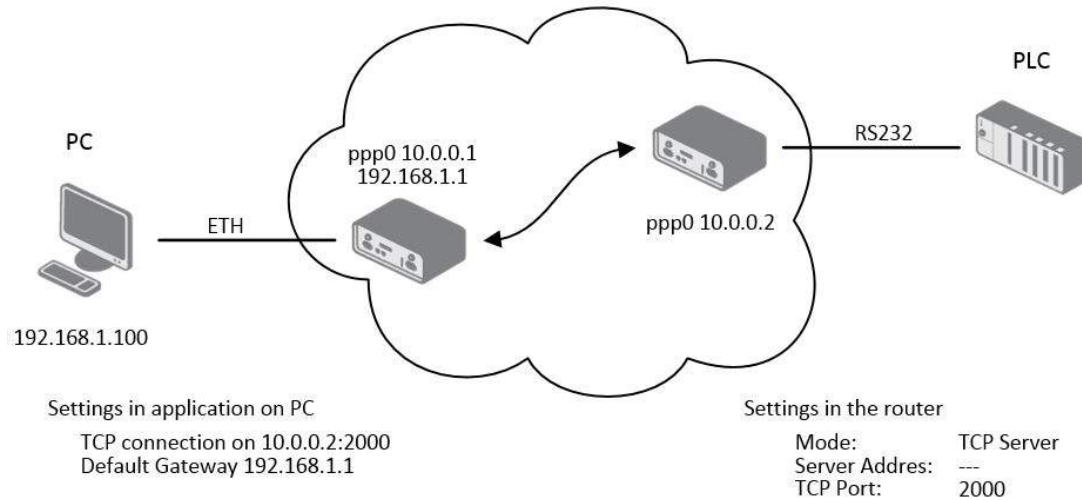
Figure 66: Example of Ethernet to serial communication
