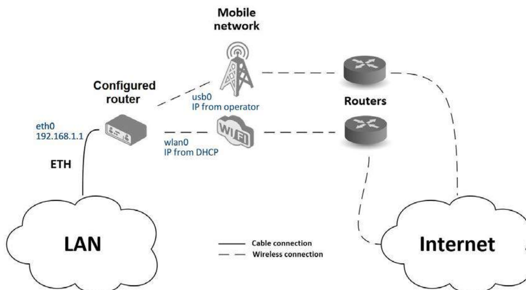
Figure 89: Backup access to the Internet – sample topology
