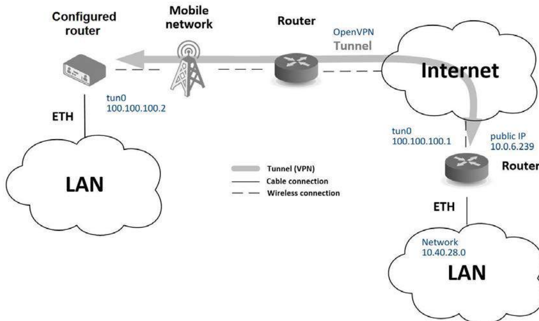
Figure 93: Secure networks interconnection – sample topology
