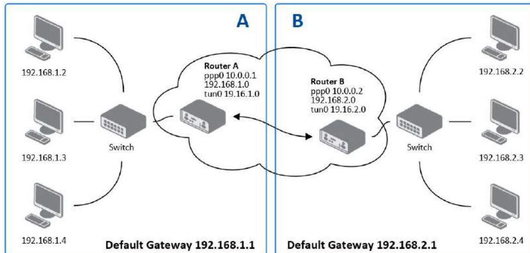
Figure 40: Topology of OpenVPN Configuration Example
