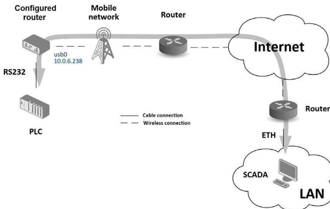
Figure 95: Serial Gateway – sample topology
