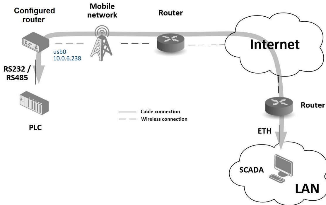
Figure 112: Serial Gateway – sample topology
