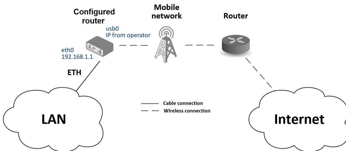
Figure 102: Access to the Internet from LAN – sample topology
