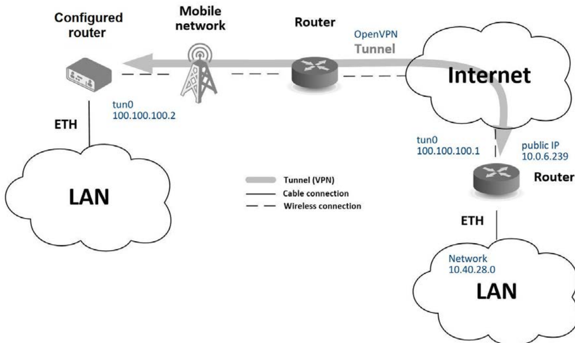
Figure 112: Secure networks interconnection – sample topology
