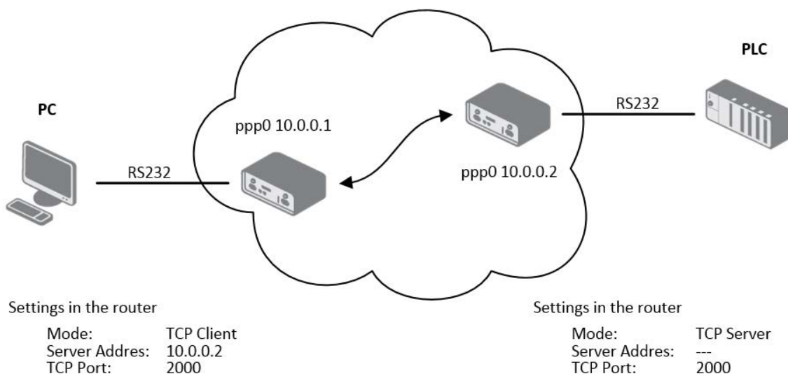
Figure 76: Example of serial interface configuration
