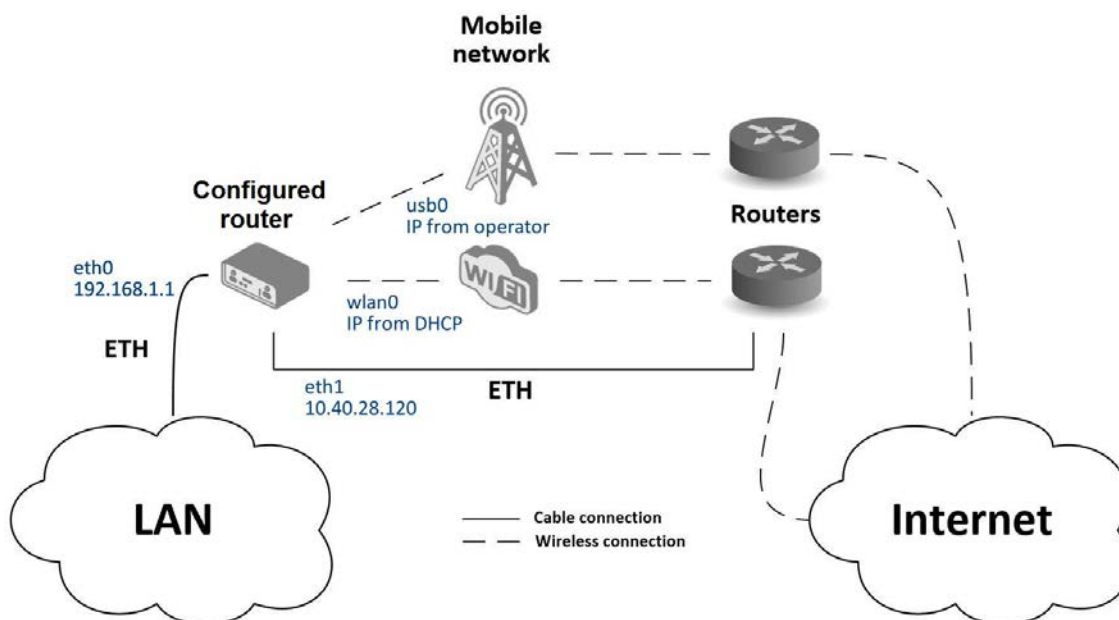
Figure 107: Backup access to the Internet – sample topology
