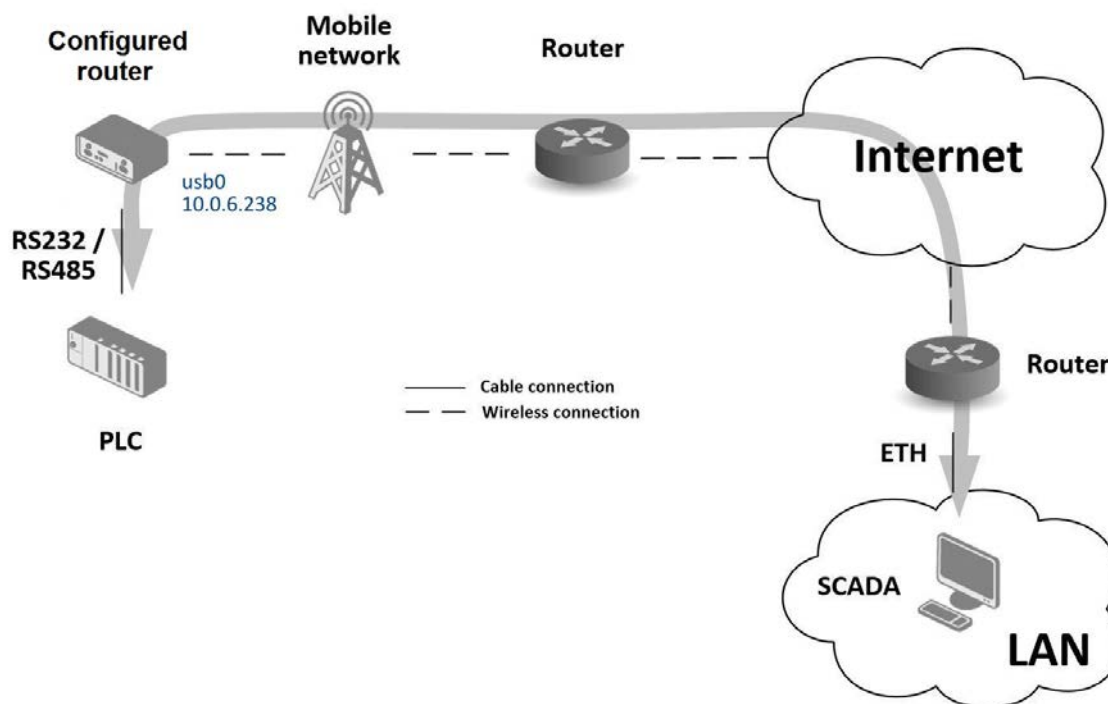
Figure 114: Serial Gateway – sample topology
